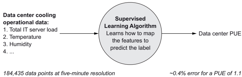
Figure 2.6 Gao's machine learning model
