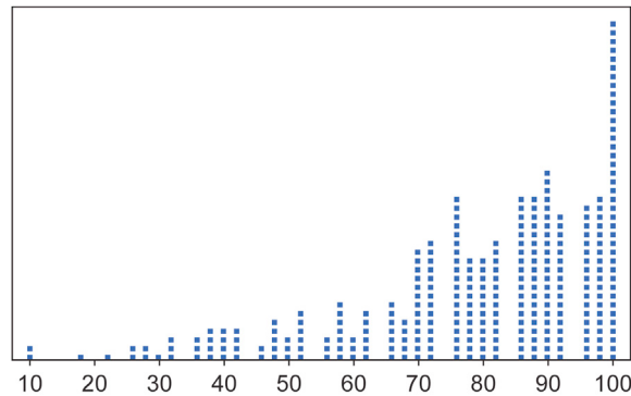
FIGURE A.9 Graph of 311 SUS scores
