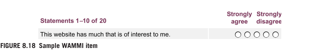
FIGURE 8.18 Sample WAMMI item
