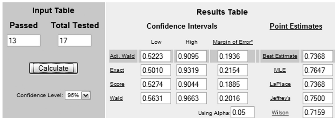
FIGURE 6.5 Result of Sample Size Estimation Example for Adjusted-Wald Binomial Confidence Interval
