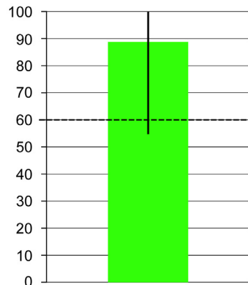
FIGURE 4.3 Sixty percent is a plausible result
