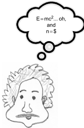
FIGURE 6.1 You Don't Have to be Einstein to Figure out the Relationship Between Sample Size and Economics
