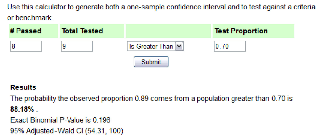
FIGURE 4.5 p and mid- p results for eight successes out of nine attempts compared to criterion of 70% success
