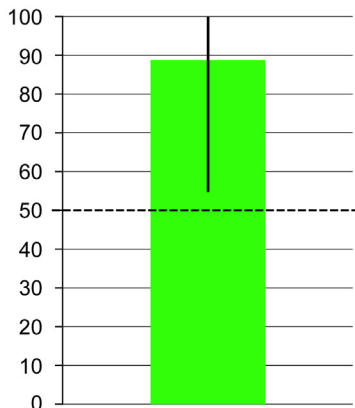
FIGURE 4.2 Fifty percent is an improbable result
