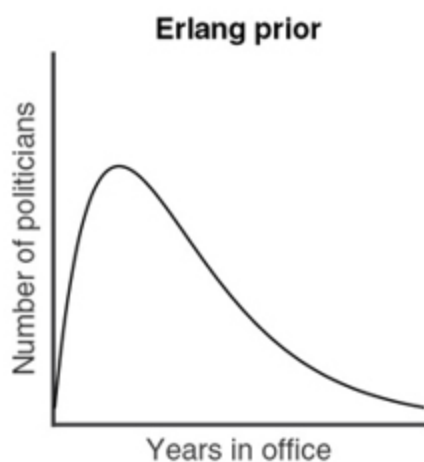
Different prior distributions and their prediction rules.
